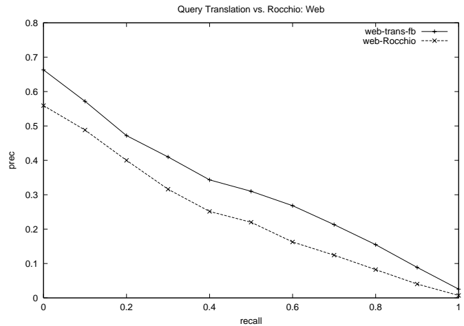
Figure 6: Precision-recall curves comparing TF-IDF with Rocchio to the query translation models. The curves for the two methods on AP89 are nearly the same, and so are not shown.
