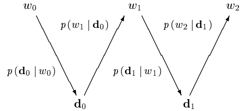
Figure 2: The Markov chain alternates between words and documents. For a given document, a word is selected according to the document language model. For a given word, a document is selected according to the posterior probability.
