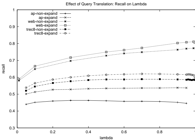
Figure 5: Effect of \lambda , the document smoothing parameter for linear interpolation. The results indicate that the improvement of the query translation model over the simple query model is fairly insensitive to the choice of \lambda .
