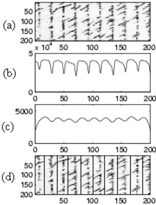
Figure 6: (a) A section of an image, (b) projection profile, (c) smoothed projection profile (d) line segmented image
