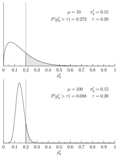
Figure 3: The effect of \mu on the probability of a below-threshold query being presented.
