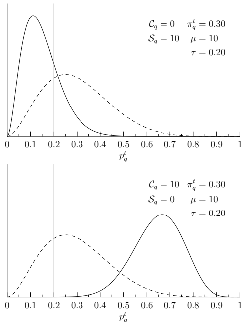
Figure 2: The effect of click information on the posterior. The prior is shown as a dashed line.
